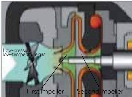
Two stage compression load adaptive capacity is better
